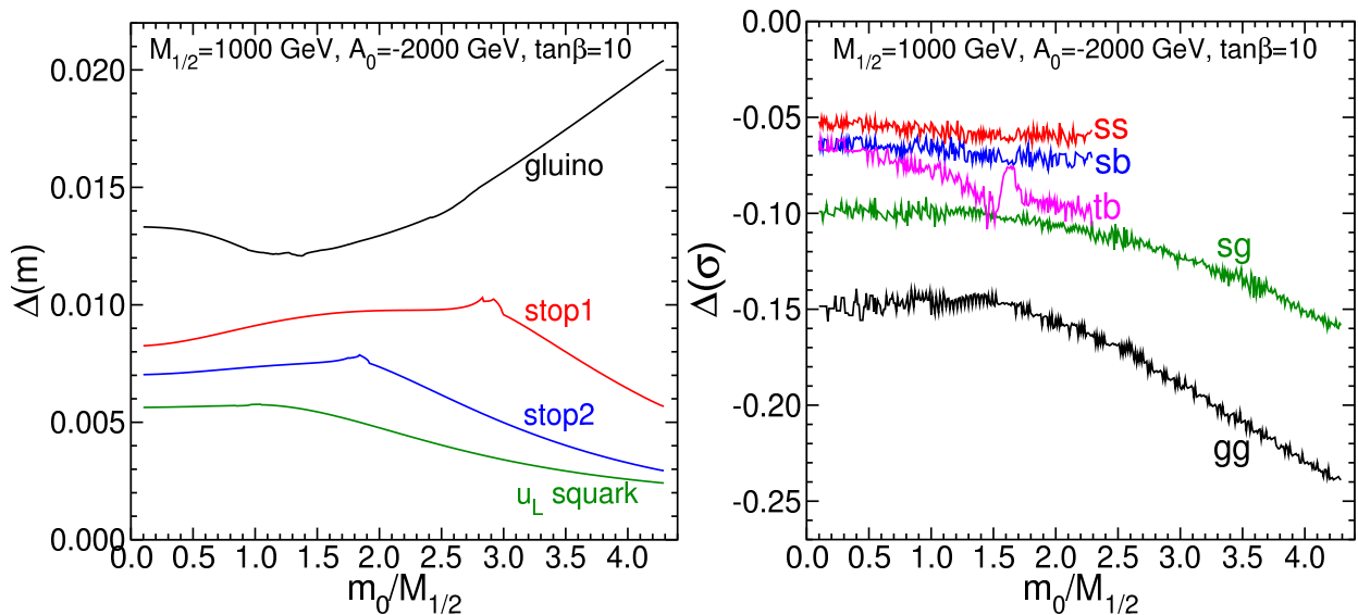
Figure 3: Effects of the 2-loop SUSYQCD corrections to sparticle pole masses (left panel) and total production cross-sections (right panel), for a line in CMSSM space with M_{1/2} = 1 \text{ TeV} , A_0 = -2 \text{ TeV} , \tan\beta = 10 and \mu > 0 . In the left panel, \Delta(m) = m_{2\text{-loop}}/m_{1\text{-loop}} - 1 , where m_{2\text{-loop}} is the pole mass calculated including the \mathcal{O}(\alpha_s^2/(16\pi^2)) terms whereas m_{1\text{-loop}} is the pole mass calculated at one-loop order. In the right panel, \Delta(\sigma) = \sigma_{2\text{-loop}}/\sigma_{1\text{-loop}} - 1 , where \sigma_{2\text{-loop}} is the 13 TeV LHC production cross-section calculated using the \mathcal{O}(\alpha_s^2/(16\pi^2)) terms in pole masses whereas \sigma_{1\text{-loop}} is the 13 TeV LHC production cross-section calculated with one-loop pole masses. The label ‘gg’ refers to gluino-gluino production, ‘sg’ to squark-gluino plus antisquark-gluino, ‘ss’ to squark-squark plus antisquark-antisquark, ‘sb’ to squark-antisquark, and ‘tb’ to stop-antistop production. The cross-sections in each case are obtained at NLL+NLO using NLL-fastv3.1-13TeV [17, 18, 19, 20, 18, 21, 22, 23, 24].
